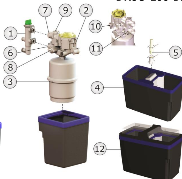
DHSO-100-BL
