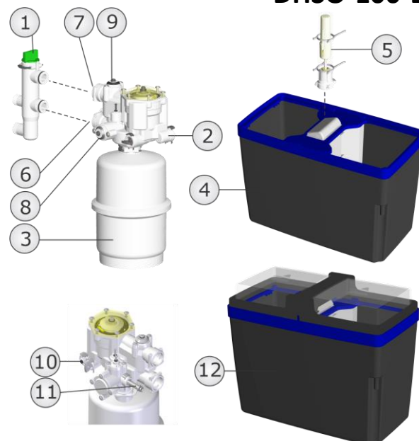
DHSO-100-BL
